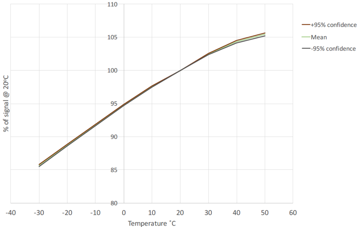
Output vs Temp
