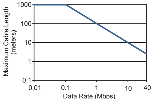
Figure 1. Maximum cable length versus data rate.
