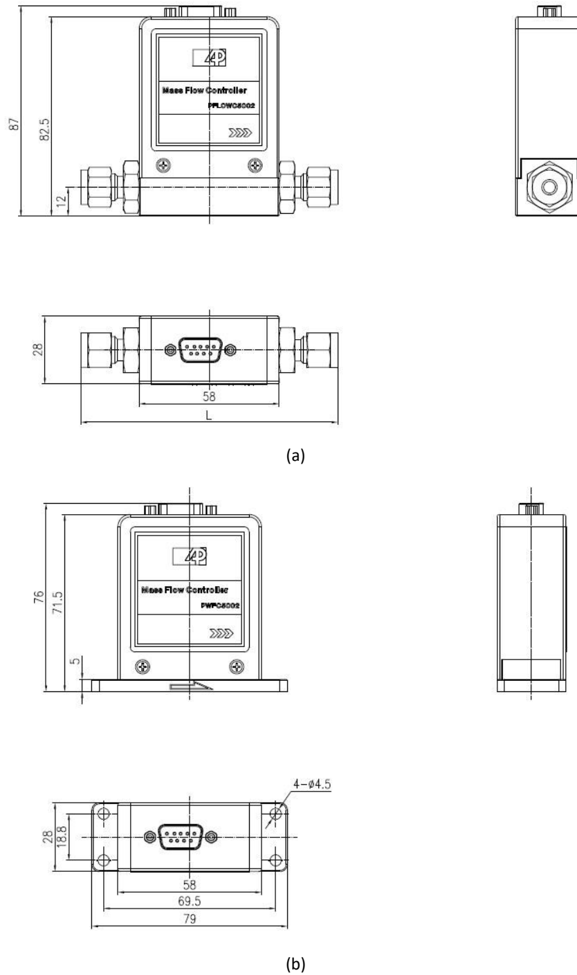
Figure 3.2: (a) PFLOW5002/5002C mechanical dimension; (b) manifold model mechanical dimensions.
