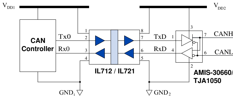
Figure 2. Isolated CAN circuit.
