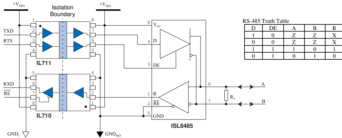
Figure 1. Isolated PROFIBUS / RS-485 circuit.
