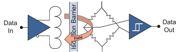
Figure 4. IL711 / IL712 / IL721 equivalent circuit (each channel).
