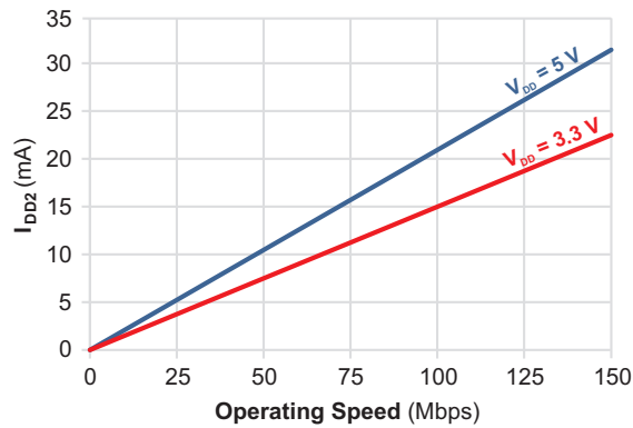
Figure 1. Supply current vs. operating speed.
