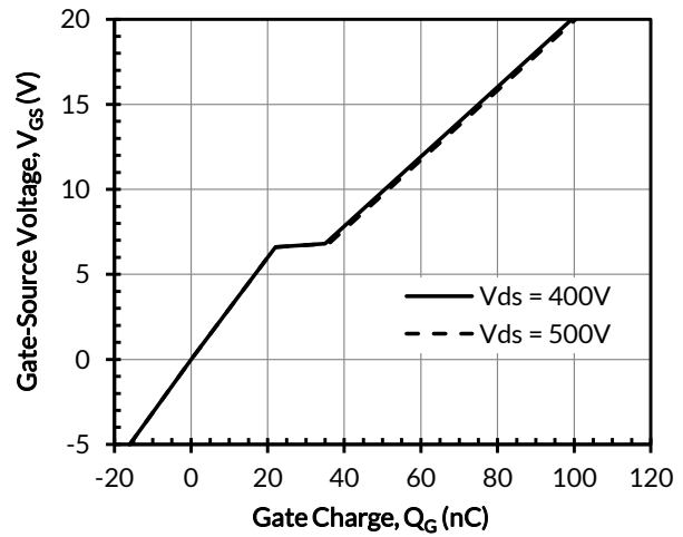
Figure 8. Typical gate charge at I_D = 60A
