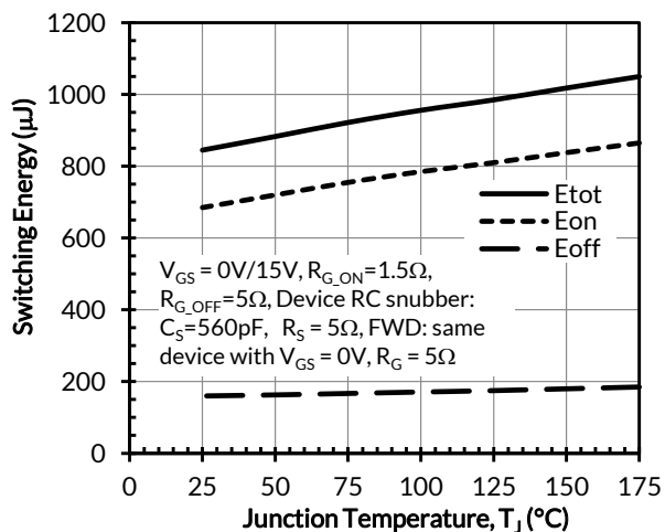
Figure 28. Clamped inductive switching energy vs. junction temperature at V_{DS} = 500V and I_D = 70A
