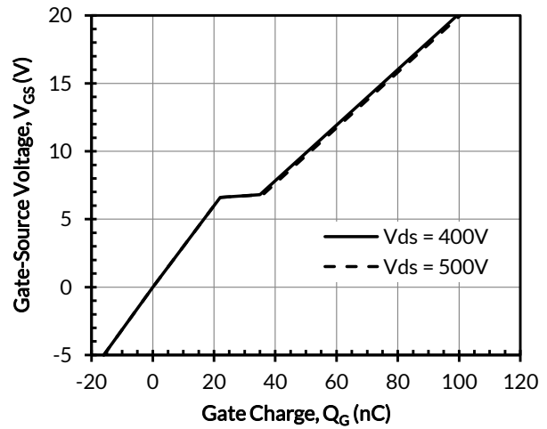
Figure 8. Typical gate charge at I_D = 70A
