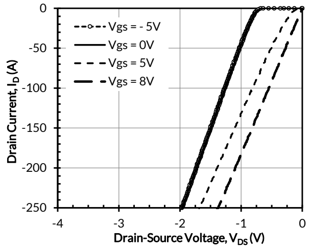
Figure 10. 3rd quadrant characteristics at T_j = 25^\circ\text{C}
