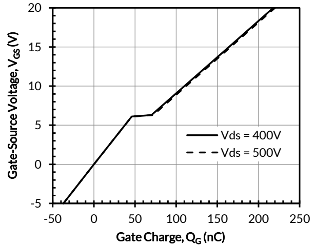
Figure 8. Typical gate charge at I_D = 80A
