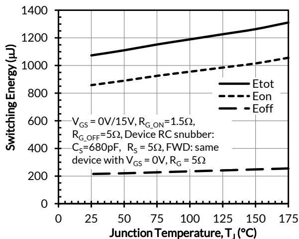
Figure 28. Clamped inductive switching energy vs. junction temperature at V_{DS} = 500V and I_D = 80A
