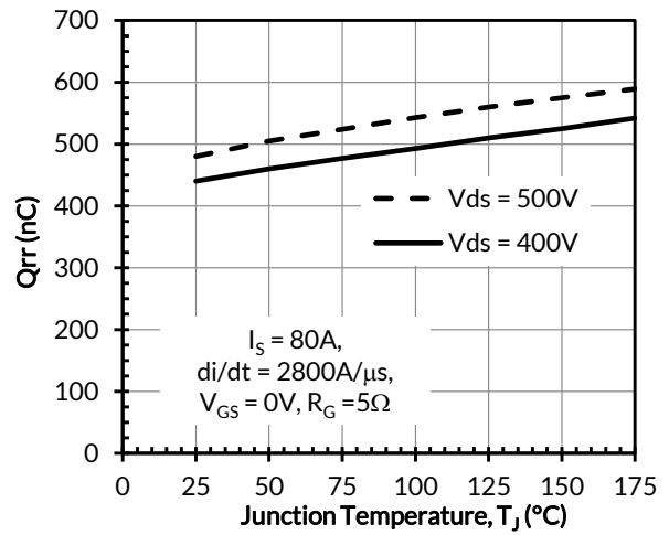
Figure 18. Reverse recovery charge Q_{rr} vs. junction temperature
