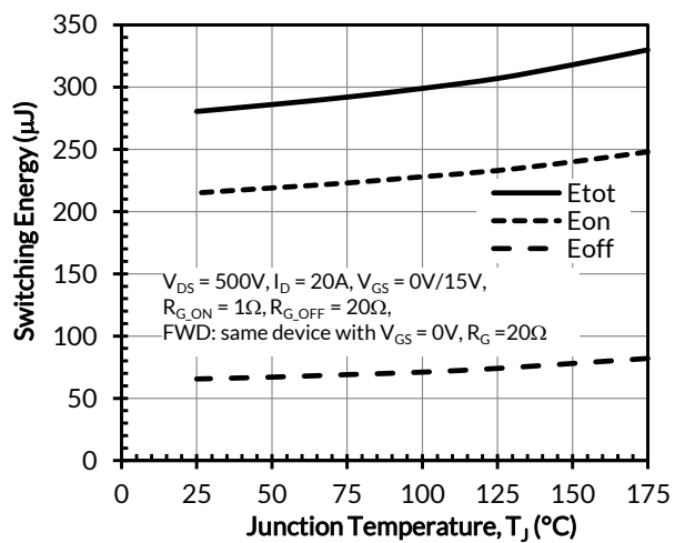
Figure 24. Clamped inductive switching energy vs. junction temperature at V_{DS}=500V and I_D = 20A
