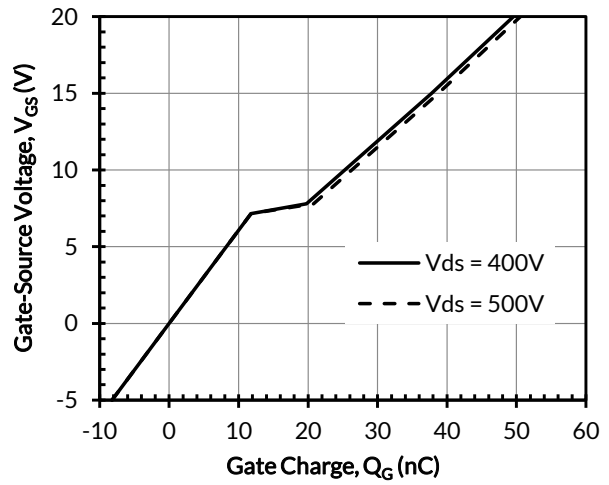
Figure 8. Typical gate charge at I_D = 20A
