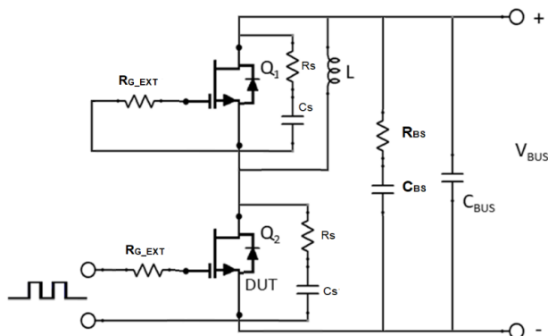
Figure 35. Schematic of the half-bridge mode switching test circuit. Note, a bus RC snubber ( R_{BS} = 5\Omega, C_{BS} = 100nF ) is used to reduce the power loop high frequency oscillations.
