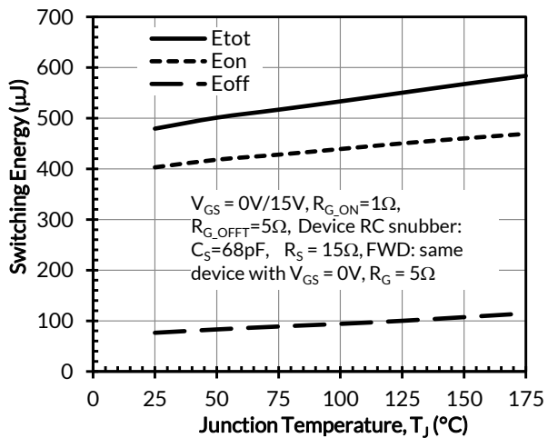
Figure 28. Clamped inductive switching energy vs. junction temperature at V_{DS} = 500V and I_D = 25A
