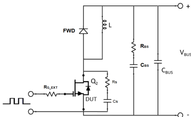
Figure 36. Schematic of the chopper mode switching test circuit. Note, a bus RC snubber ( R_{BS} = 5\Omega, C_{BS} = 100nF ) is used to reduce the power loop high frequency oscillations.
