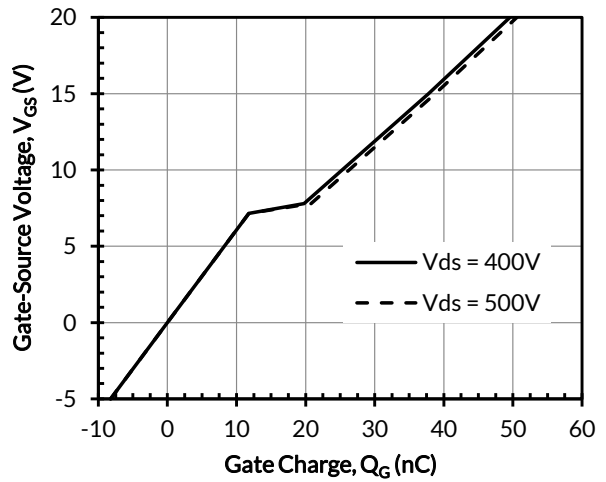
Figure 8. Typical gate charge at I_D = 25A
