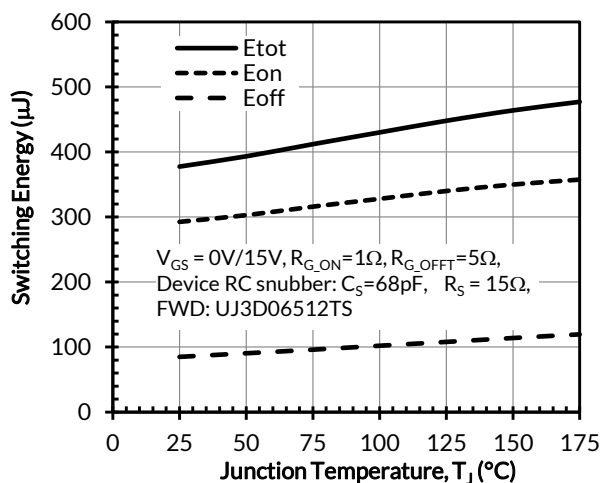
Figure 34. Clamped inductive switching energy vs. junction temperature at V_{DS} = 500V and I_D = 25A
