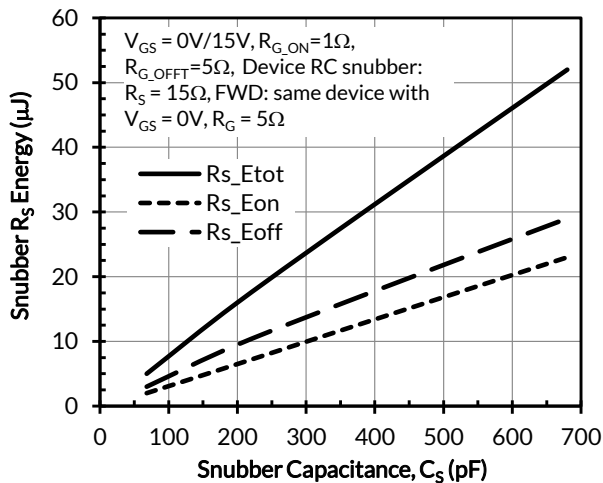
Figure 26. RC snubber energy losses vs. snubber capacitance C_s at V_{DS} = 400V, I_D = 25A, and T_J = 25^\circ C
