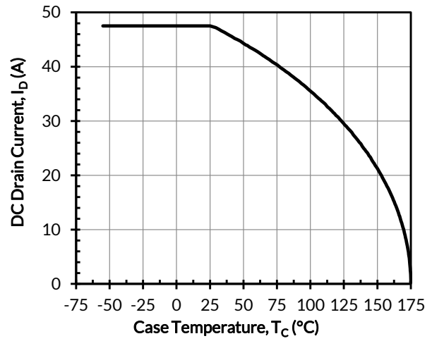
Figure 14. DC drain current derating
