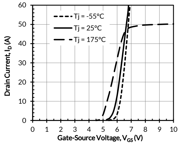
Figure 6. Typical transfer characteristics at V_{DS} = 5V
