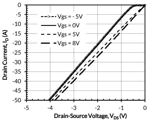
Figure 11. 3rd quadrant characteristics at T_J = 175^\circ\text{C}
