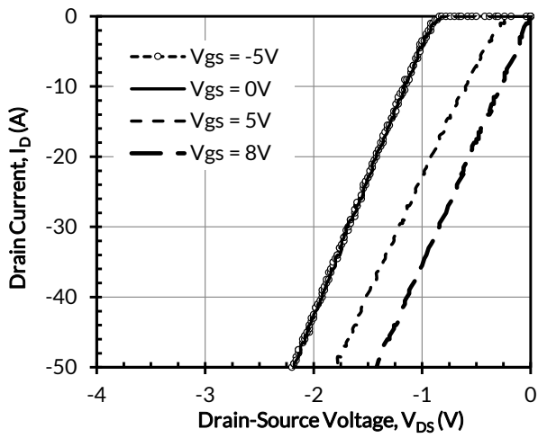
Figure 9. 3rd quadrant characteristics at T_J = -55^\circ\text{C}
