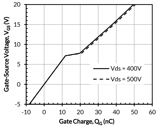
Figure 8. Typical gate charge at I_D = 30A
