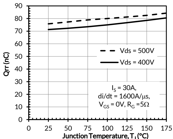
Figure 18. Reverse recovery charge Q_{rr} vs. junction temperature
