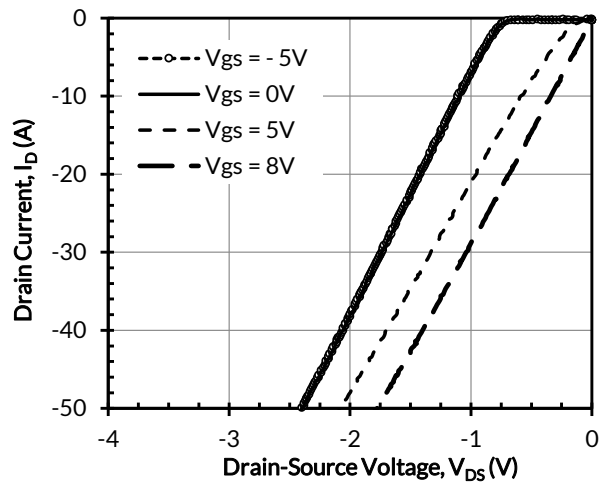
Figure 10. 3rd quadrant characteristics at T_J = 25^\circ\text{C}
