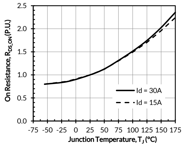
Figure 4. Normalized on-resistance vs. temperature at V_{GS} = 12\text{V}
