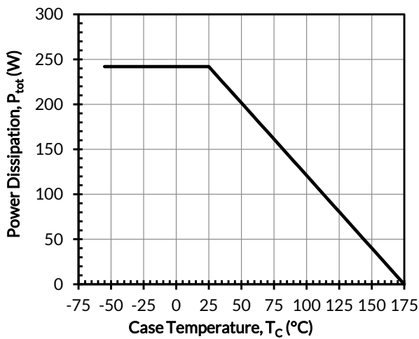
Figure 15. Total power dissipation
