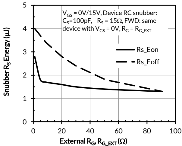
Figure 24. RC snubber energy losses vs. R_{G,EXT} at V_{DS} = 400V , I_D = 30A , and T_J = 25^\circ C
