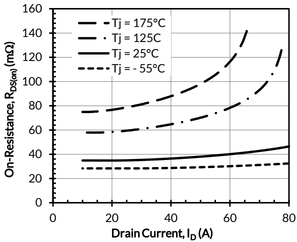
Figure 5. Typical drain-source on-resistances at V_{GS} = 12V
