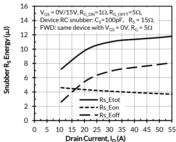
Figure 22. RC snubber energy losses vs. drain current at V_{DS} = 500V and T_J = 25^\circ C
