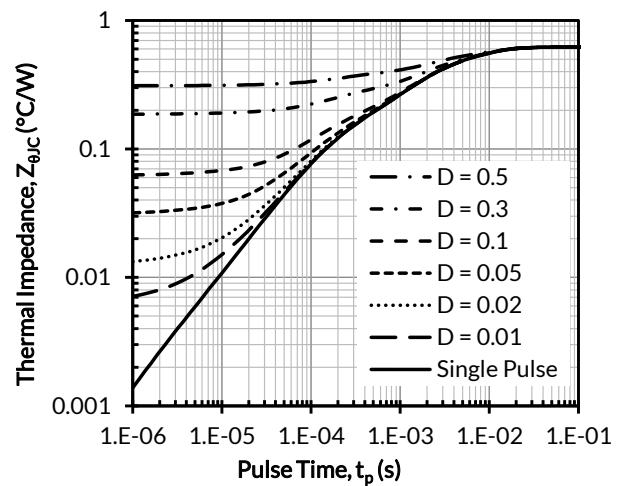
Figure 16. Maximum transient thermal impedance
