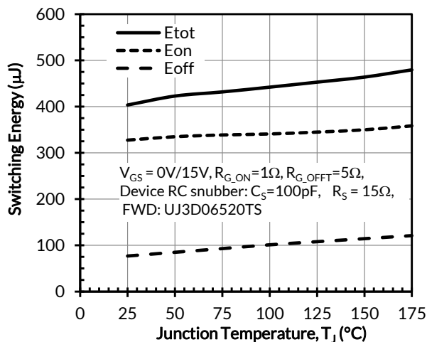
Figure 34. Clamped inductive switching energy vs. junction temperature at V_{DS} = 500V and I_D = 30A
