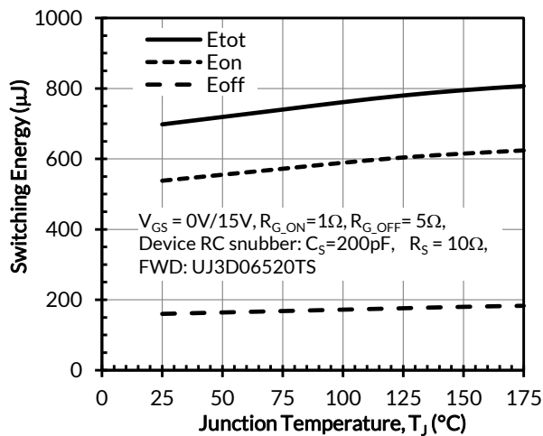
Figure 34. Clamped inductive switching energy vs. junction temperature at V_{DS} = 500V and I_D = 40A
