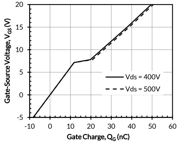
Figure 8. Typical gate charge at I_D = 40A
