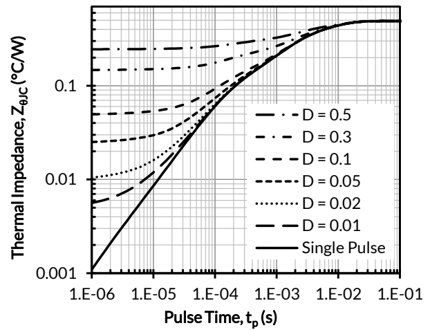
Figure 16. Maximum transient thermal impedance
