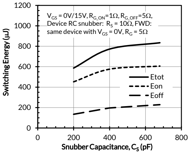
Figure 25. Clamped inductive switching energies vs. snubber capacitance C_s at V_{DS} = 400V, I_D = 40A , and T_J = 25^\circ\text{C}
