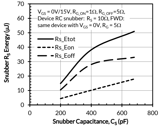
Figure 26. RC snubber energy losses vs. snubber capacitance C_s at V_{DS} = 400V, I_D = 40A , and T_J = 25^\circ\text{C}
