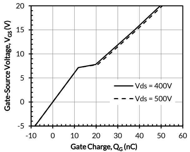
Figure 8. Typical gate charge at I_D = 50A
