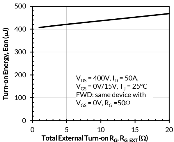
Figure 21. Clamped inductive switching turn-on energy vs. R_{G,EXT\_ON}
