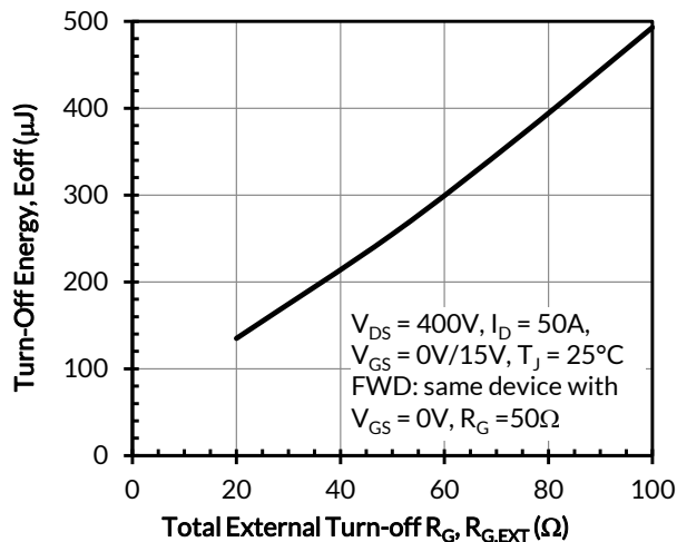
Figure 22. Clamped inductive switching turn-off energy vs. R_{G,EXT\_OFF}
