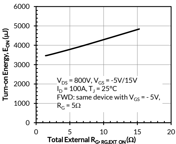
Figure 19. Clamped inductive switching turn-on energy vs. R_{G,EXT,ON}
