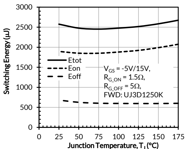
Figure 24. Clamped inductive switching energy vs. junction temperature at V_{DS} = 800V and I_D = 100A
