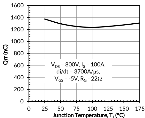
Figure 22. Reverse recovery charge Q_{rr} vs. junction temperature
