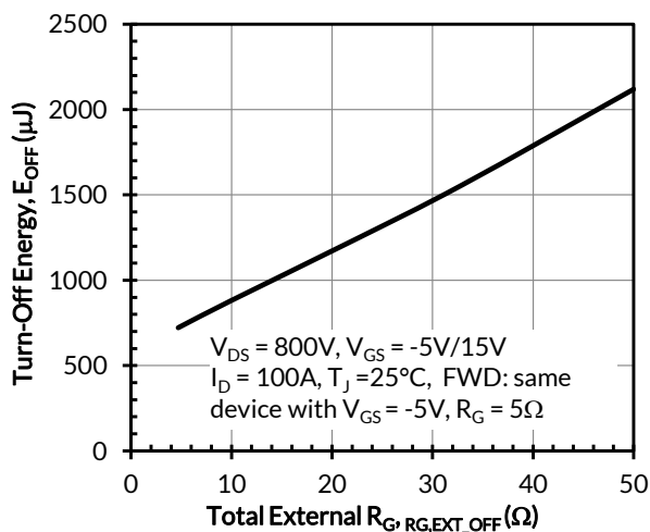
Figure 20. Clamped inductive switching turn-off energy vs. R_{G,EXT,OFF}
