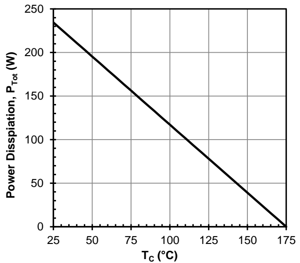
Figure 4 Power dissipation
