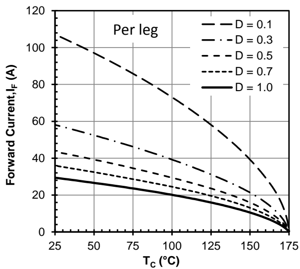
Figure 5 Diode forward current per leg
