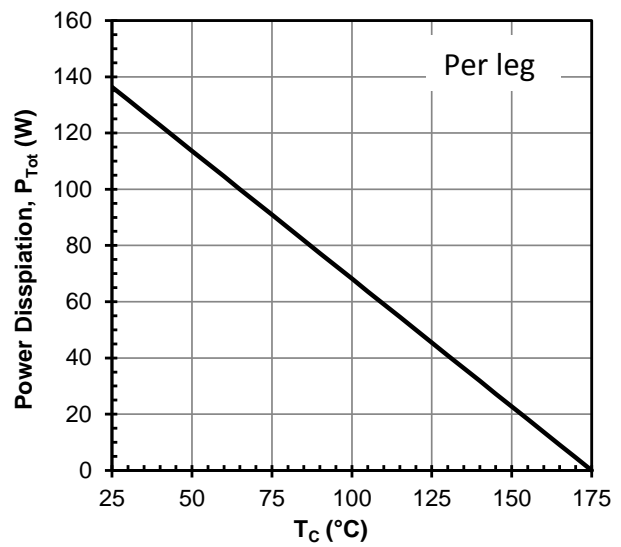
Figure 4 Power dissipation per leg
