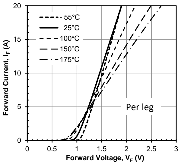
Figure 1 Typical forward characteristics per leg
