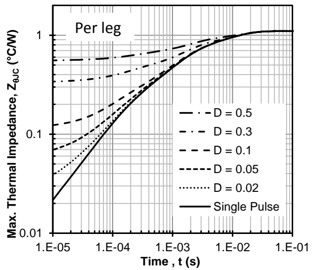
Figure 6 Maximum transient thermal impedance per leg
