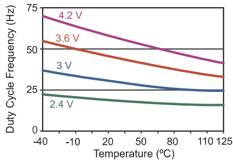
Figure 13. Typical update frequency versus temperature (ADL1xx).
