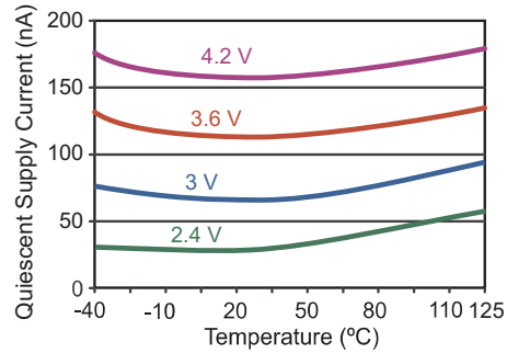
Figure 10. Typical supply current versus temperature (ADL1xx).
