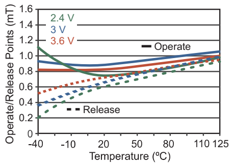
Figure 9. Typical magnetic operate point versus temperature (ADLx25).
