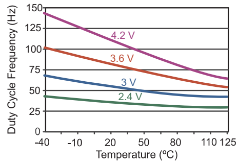
Figure 14. Typical update frequency versus temperature (ADL0xx).
