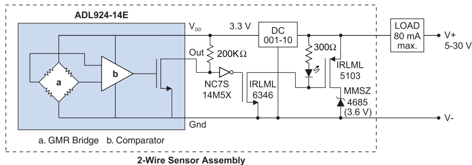
Figure 4. Typical two-wire circuit.
