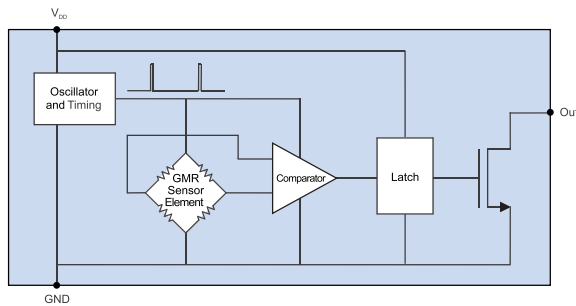
ADL0xx (duty-cycled)
