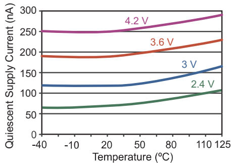
Figure 11. Typical supply current versus temperature (ADL0xx).
