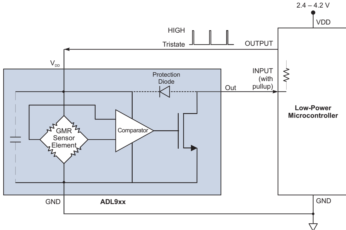
Figure 5. External duty cycling using a microcontroller.
