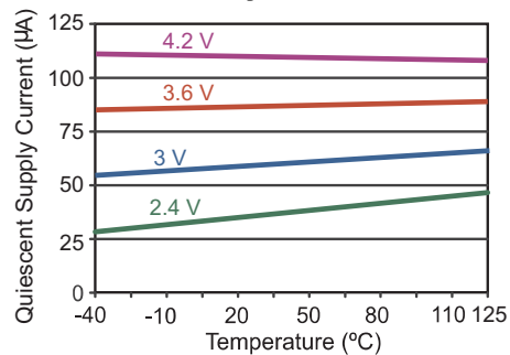
Figure 12. Typical supply current versus temperature (ADL9xx).
