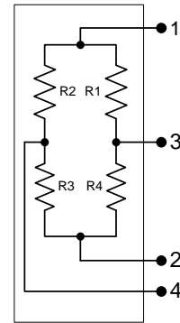
Equivalent Circuit
