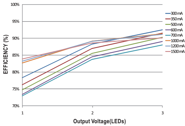
Fig-1 12VDC input, 1-3 LEDs(Vf=3V)
