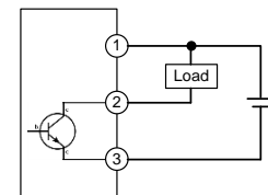
Connection Diagram
