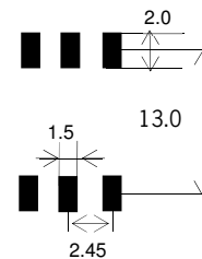
Foot print
