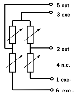
Internal circuit
