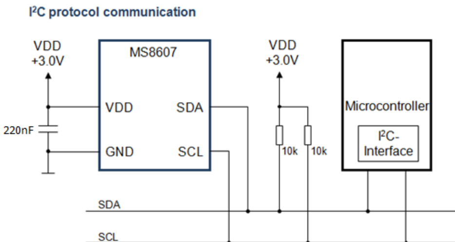
Figure 9: Typical application circuit
