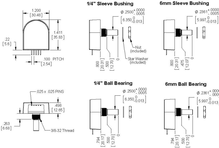
S1 Optical Shaft Encoder Drawing
